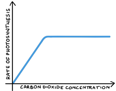
Graph of CO 2 concentration against rate of photosynthesis
