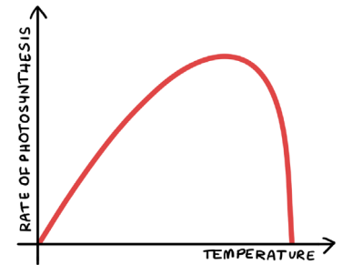
Graph of temperature against rate of photosynthesis
