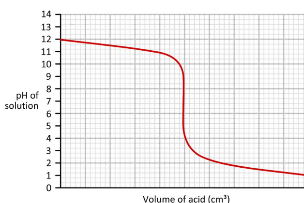
A pH graph showing an acid added to an alkali
