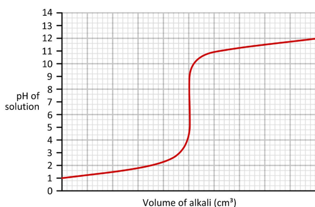
A pH graph showing an alkali added to an acid
